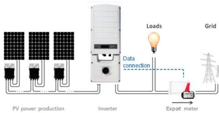
Figure 2: Typical installation with export meter
