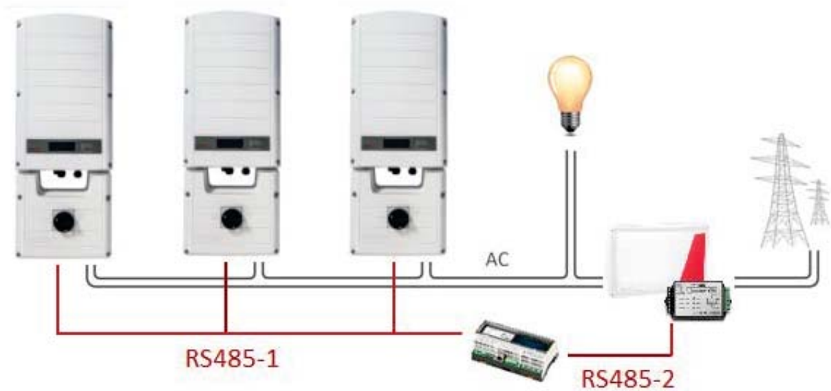
Figure 5: Multi-inverter connection with CCG
