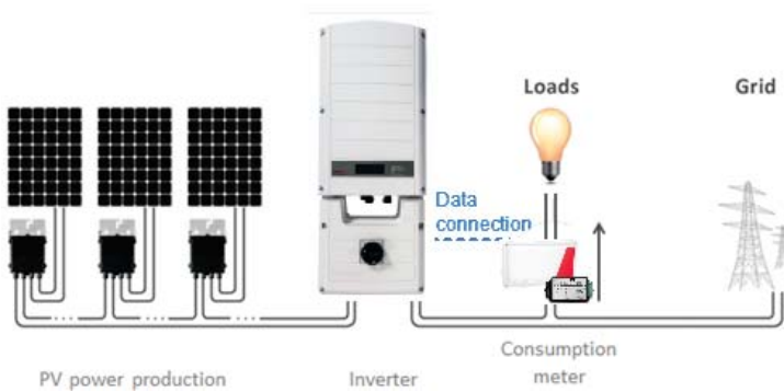
Figure 3: Typical installation with consumption meter
