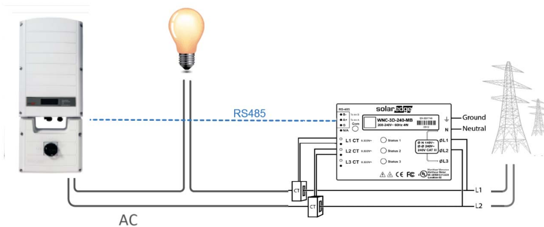
Figure 4: Single-inverter connection
