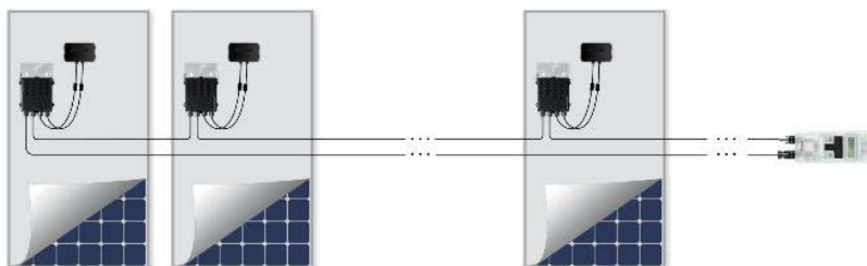
Figure 9: SolarEdge Key connection
