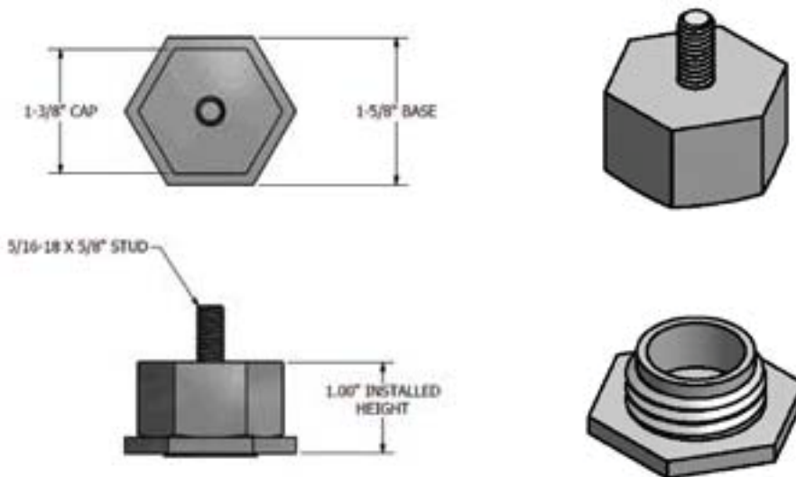
Dimensioned Metal Roof Base Assembly
