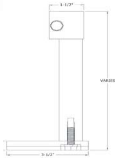
Dimensioned Standoff Assembly
