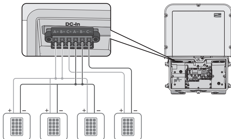
Figure 10 : Connection overview for "4-String-Operation"
