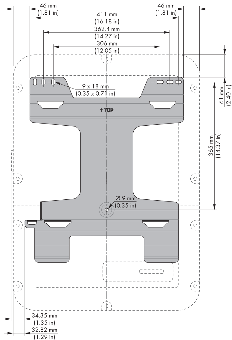
Figure 3 : Position of the anchoring points
