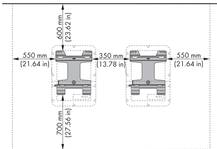
Figure 4 : Recommended clearances
