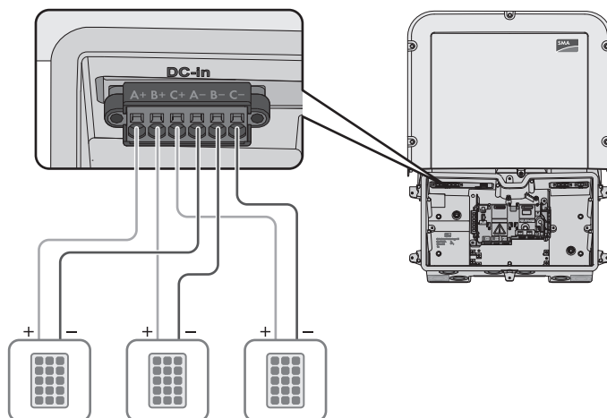
Figure 9 : Connection overview for normal operation
