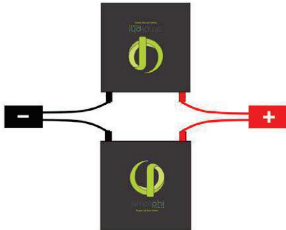
Figure 3.0 – Two PHI 3.5 Batteries in Parallel
