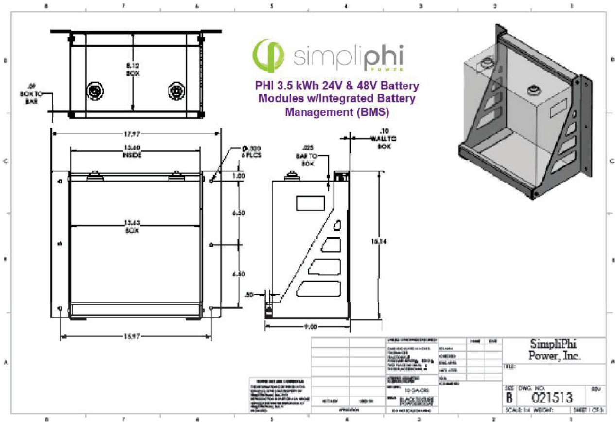
Figure 2.0 – Mounting Bracket Assembly
