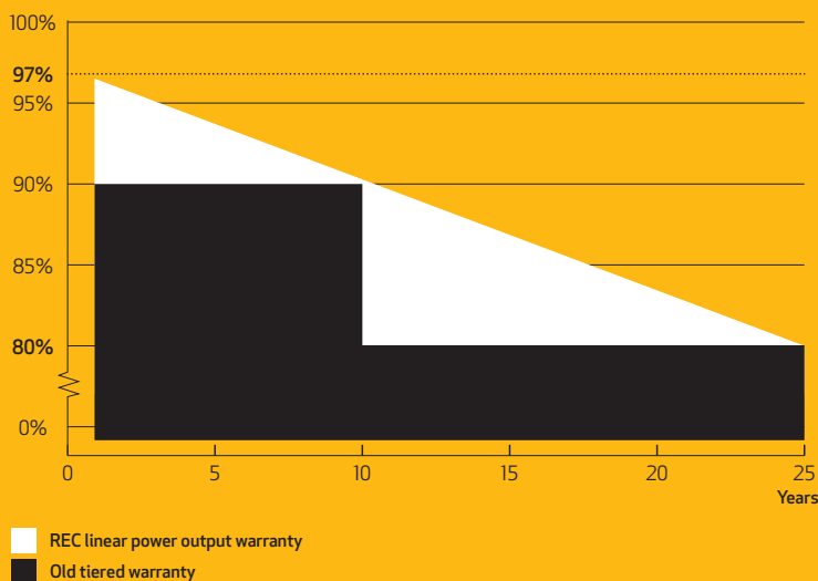
Guaranteed solar panel performance Name plate power
