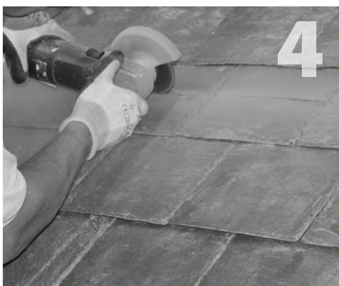
Using a cutoff wheel in a grinder, score the slate above the mounting area at 4 inches above the center of the QBase location. In step 5, you will remove the slate below the score line, which will allow you to slide the flashing up under the remaining slate in step 10.
