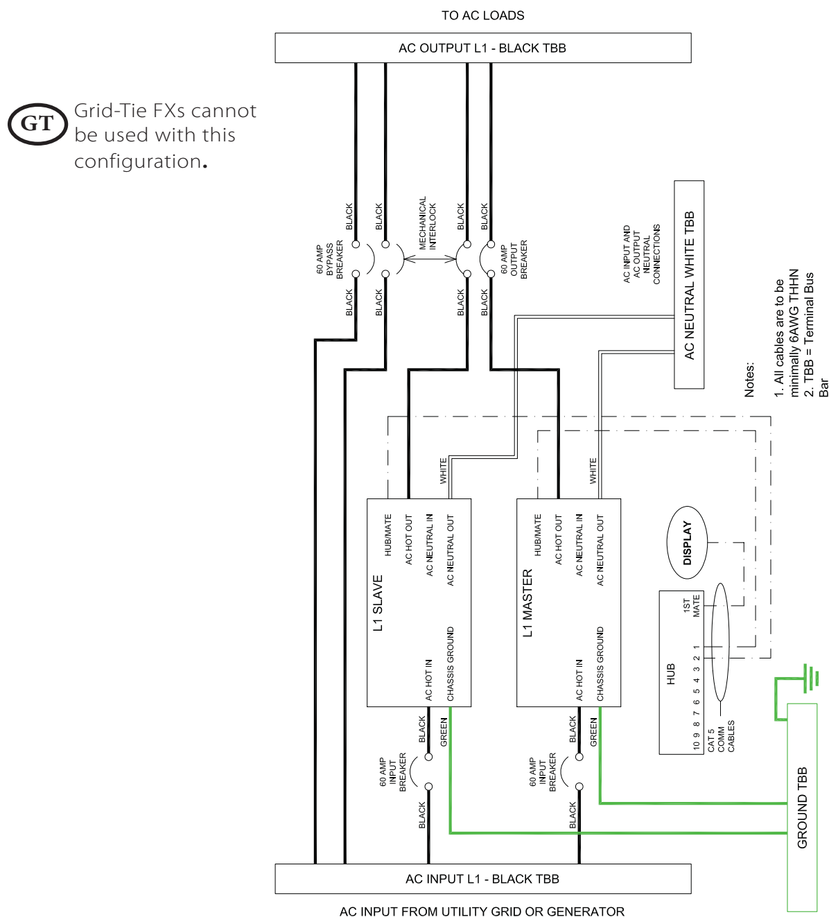
Parallel/Dual System with Two FXs
