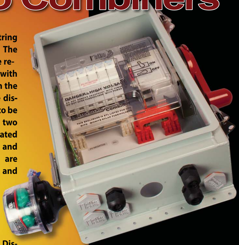
SHOWN ABOVE Six String 125 Amp/600V Disconnecting Combiner Model: MNPV6HV
