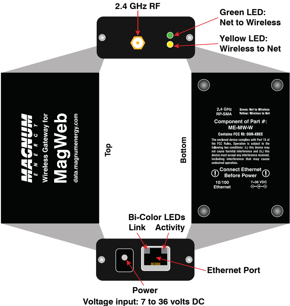
Figure 4-1, Wireless Gateway LED Diagram
