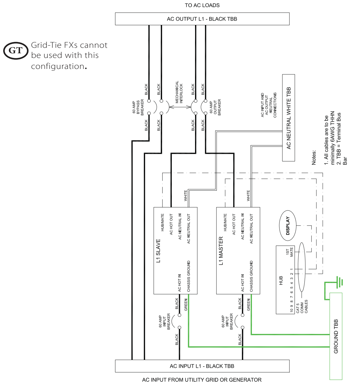
Parallel/Dual System with Two FXs
