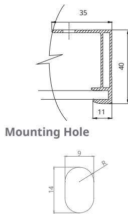
Frame Cross Section A-A
