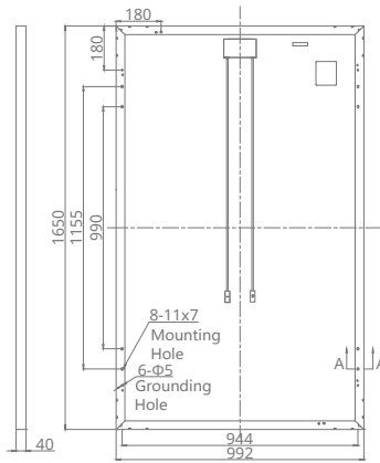
Mounting Hole
