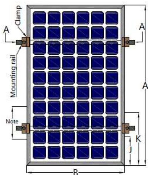
Figure 5: Installation of clamps on long side of frames
