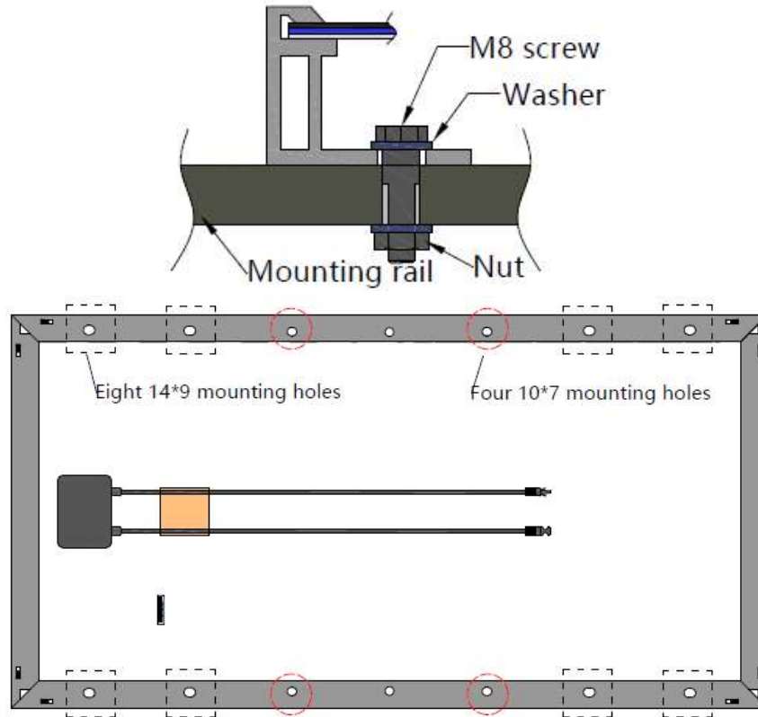
Figure 3: PV module installed with Bolt fitting method
