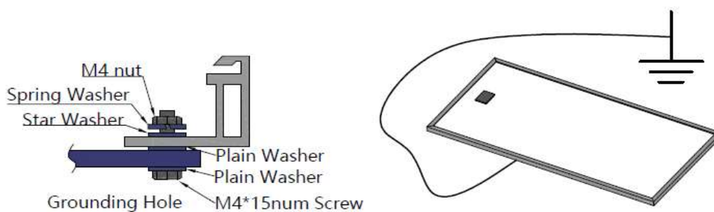
Figure 8: Ground installation of PV modules
