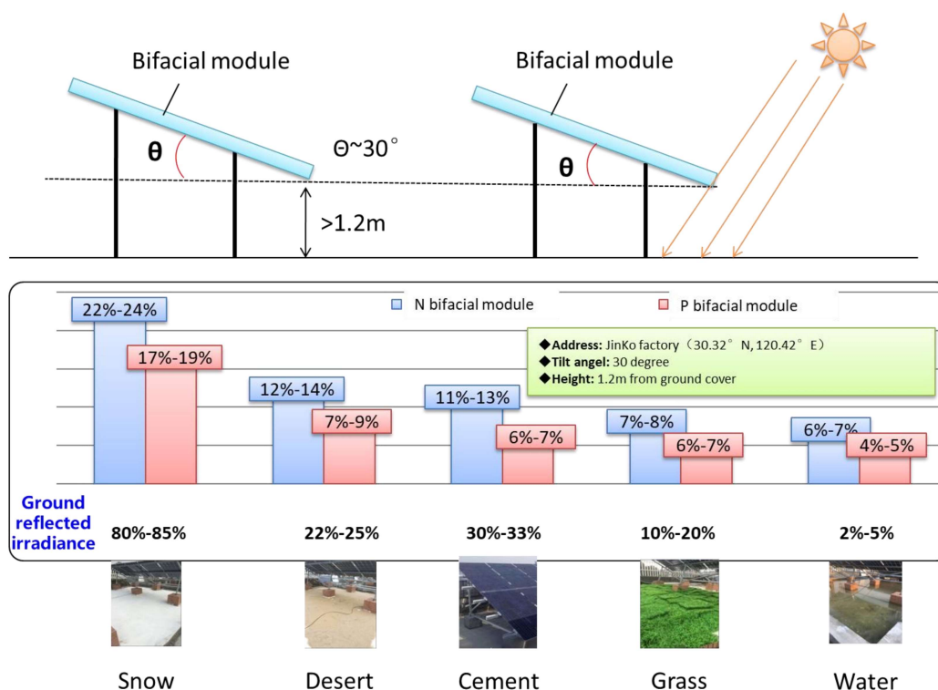
Figure2: PV module installed on different ground covers
